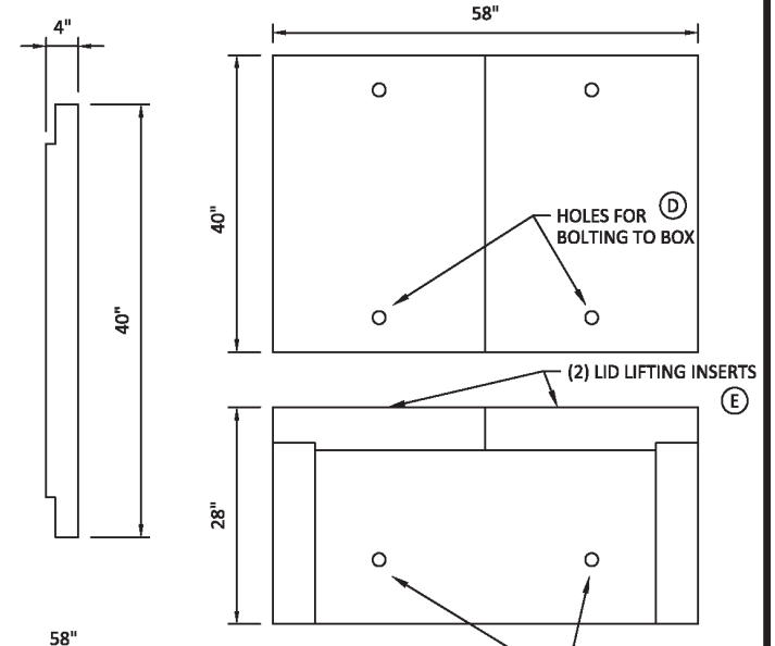
FIGURE 14B: LIDS FOR SMALL PULL AND SPLICE BOX
