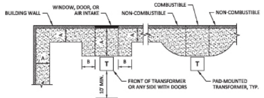
FIGURE 1 ALLOWABLE CLEARANCES
