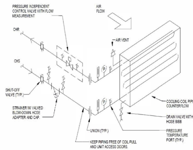
COIL PIPING SCHEMATIC
