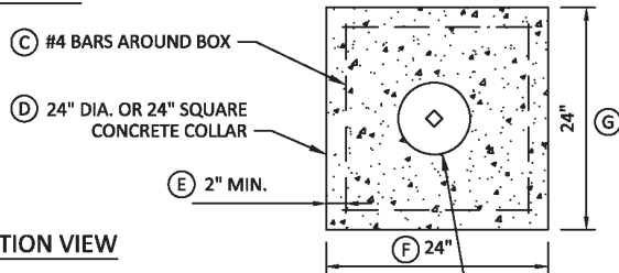
RW - FIGURE 03: LOCATING WIRE TERMINAL
