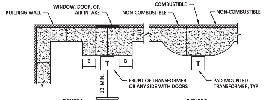
FIGURE 1 ALLOWABLE CLEARANCES
