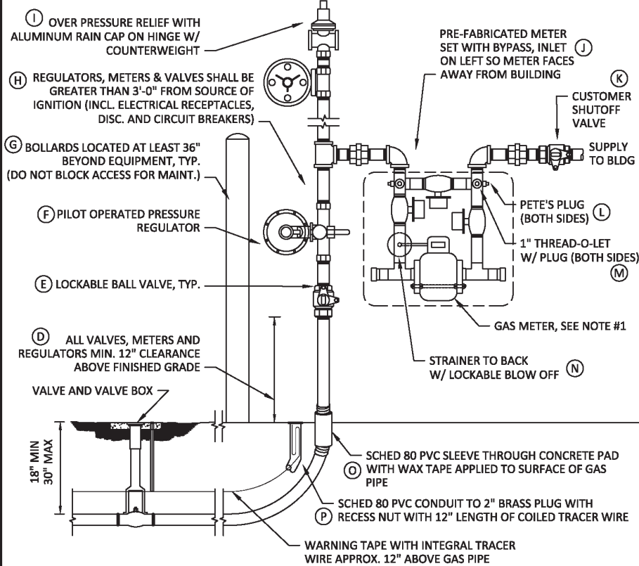
NATURAL GAS - FIGURE 06: SINGLE ROTARY GAS METER DETAIL Rev. 7/1/2019
