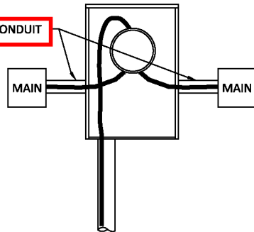
UNACCEPTABLE CONFIGURATION
