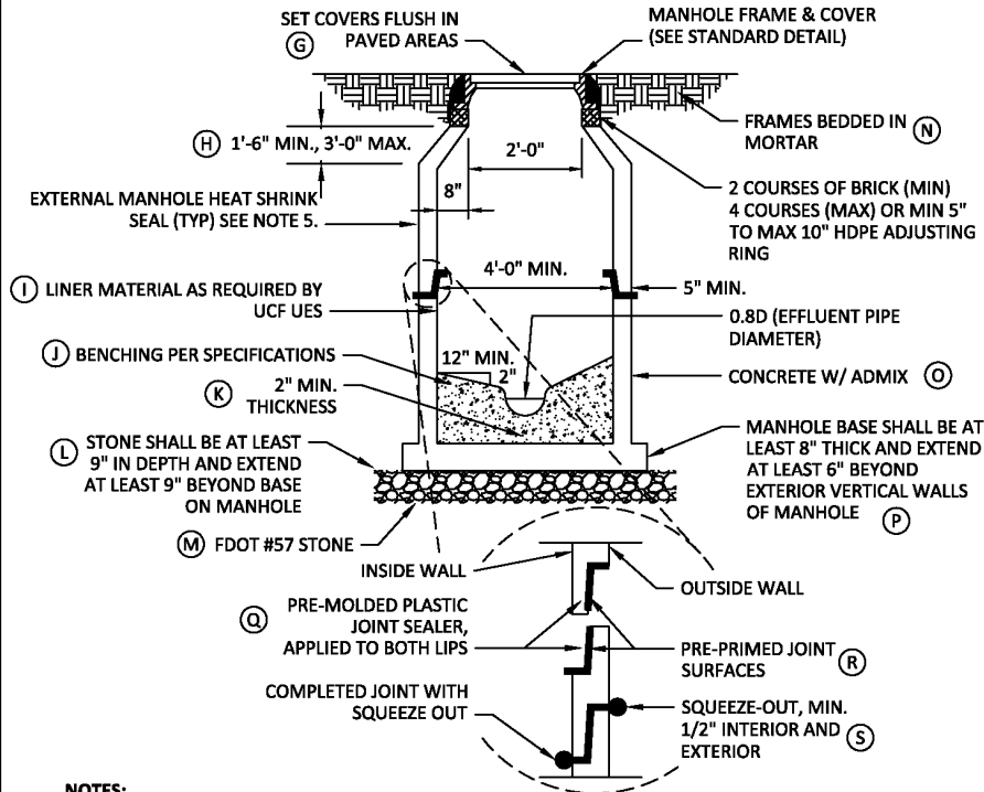
WW - FIGURE 08: PRECAST CONCRETE MANHOLE
