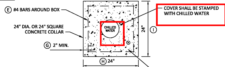
CHW - FIGURE 04: VALVE & VALVE BOX DETAIL
