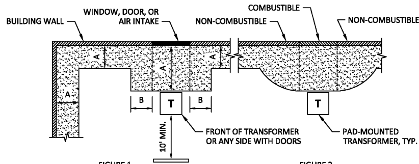
FIGURE 1 ALLOWABLE CLEARANCES
