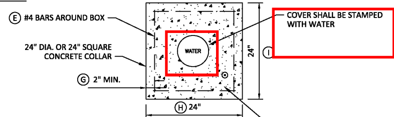
DW - FIGURE 04: VALVE & VALVE BOX DETAIL
