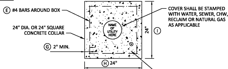
NATURAL GAS - FIGURE 04: VALVE & VALVE BOX DETAIL
