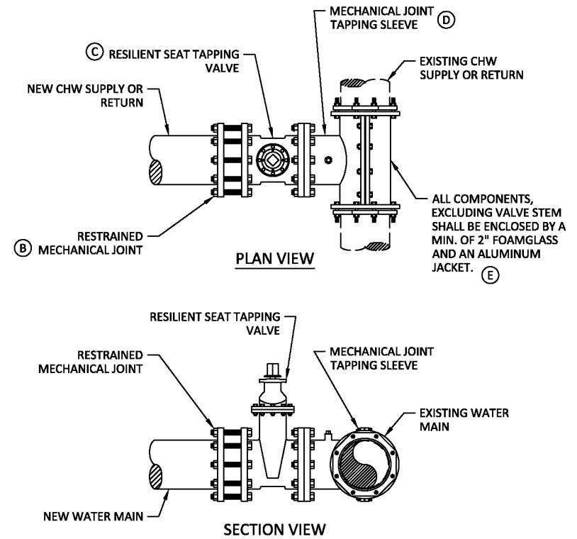
CHW - FIGURE 07: CHILLED WATER WET TAP
