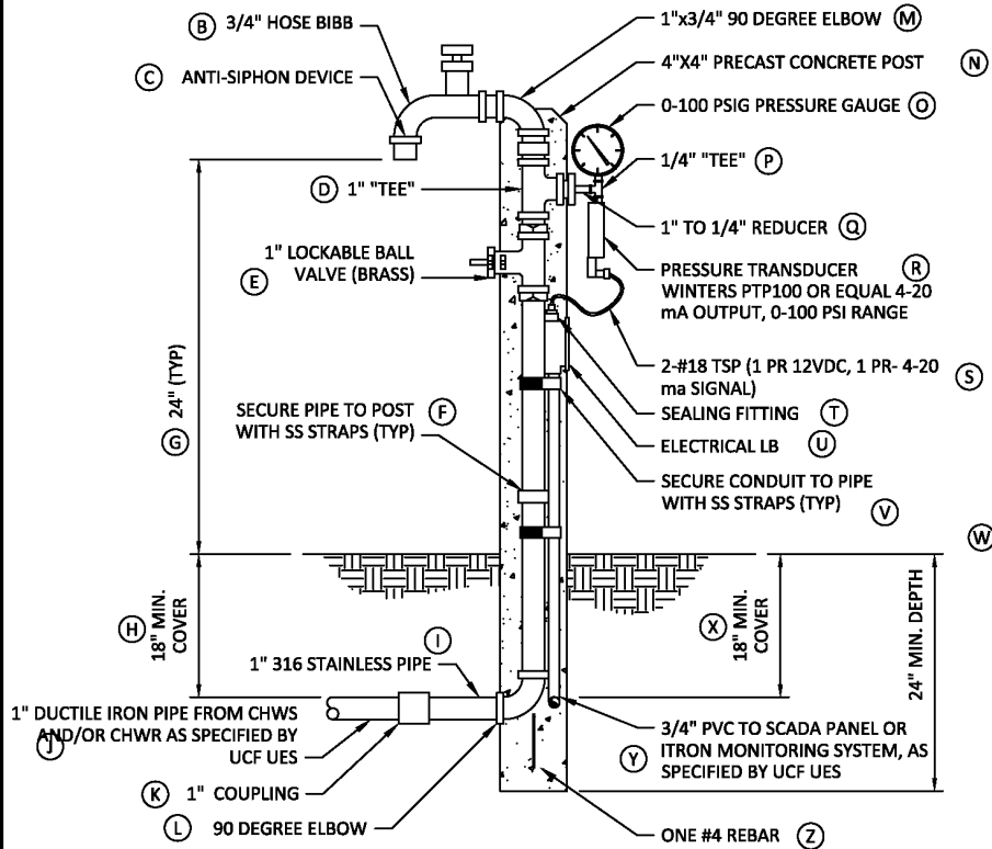
CHW - FIGURE 06: CHILLED WATER REMOTE PRESSURE AND SAMPLING POINT
