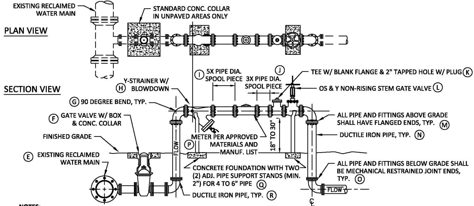
CHW - FIGURE 08: 3" AND LARGER RECLAIM MAKE-UP WATER METER
