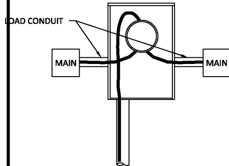
UNACCEPTABLE CONFIGURATION
