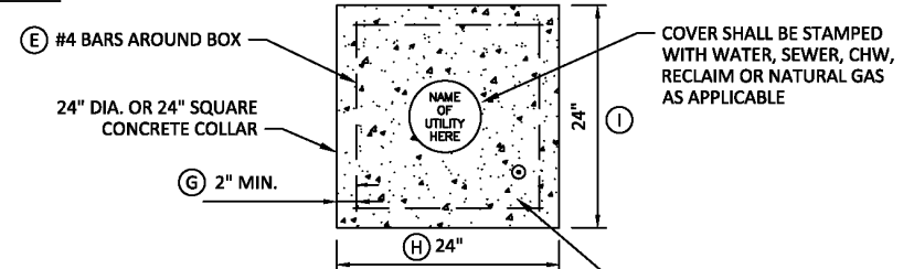
CHW - FIGURE 04: VALVE & VALVE BOX DETAIL
