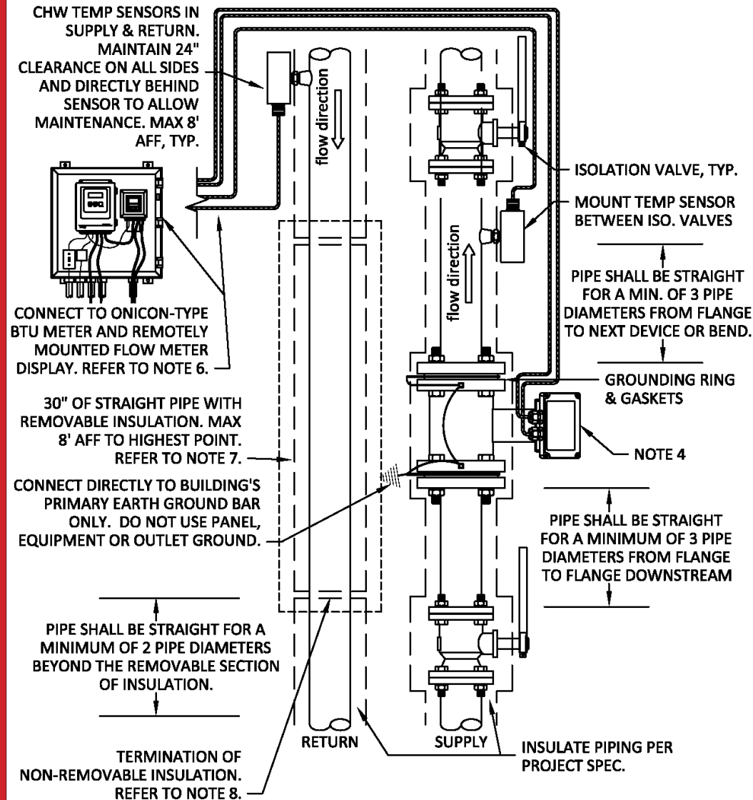
CHW - FIGURE 05A: BTU METER INSTALLATION FOR NON-CONDUCTIVE PIPE
