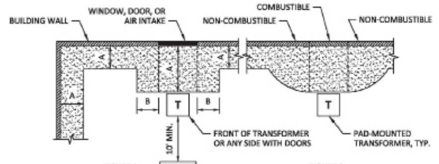
FIGURE 13: PAD MOUNTED TRANSFORMER CLEARANCES FROM BUILDINGS
