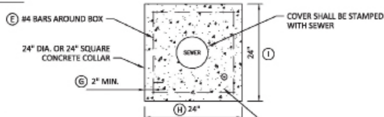
WW - FIGURE 04: VALVE &amp; VALVE BOX DETAIL
