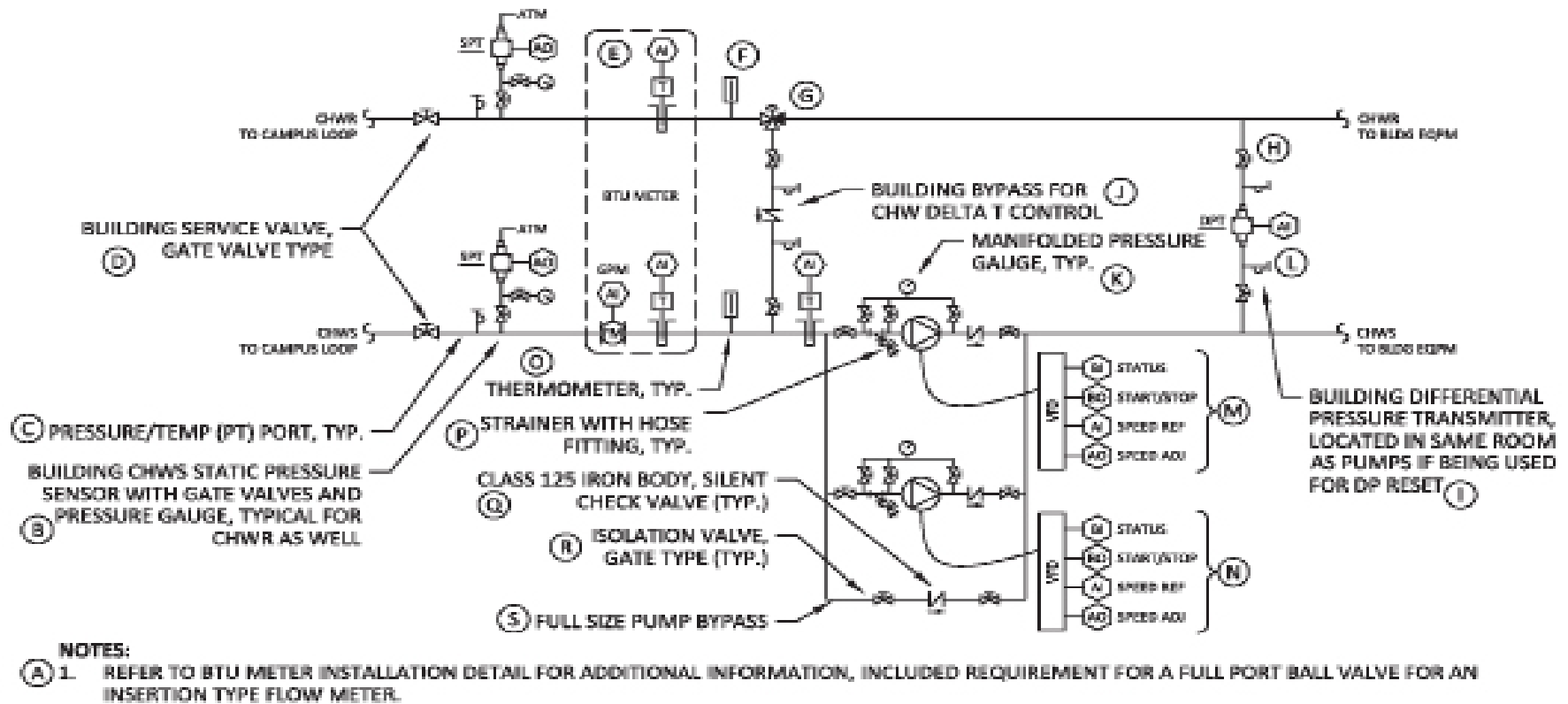
CHW - FIGURE 07: TERTIARY PUMPING SYSTEM
