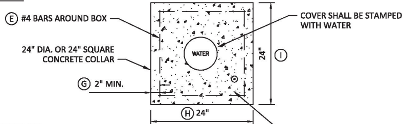
DW - FIGURE 04: VALVE & VALVE BOX DETAIL
