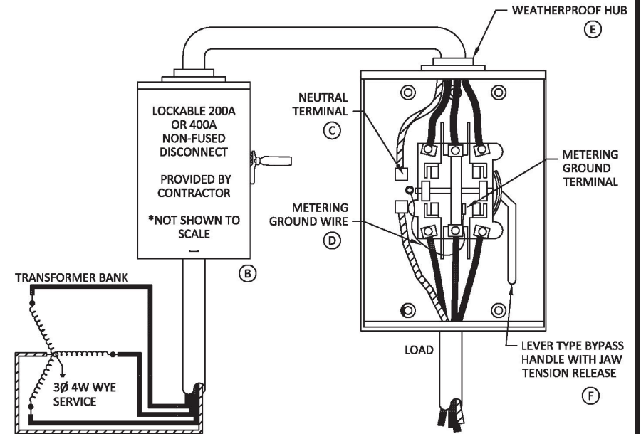
FIGURE 04D: METER BASE FORM 16S WIRING DIAGRAM
