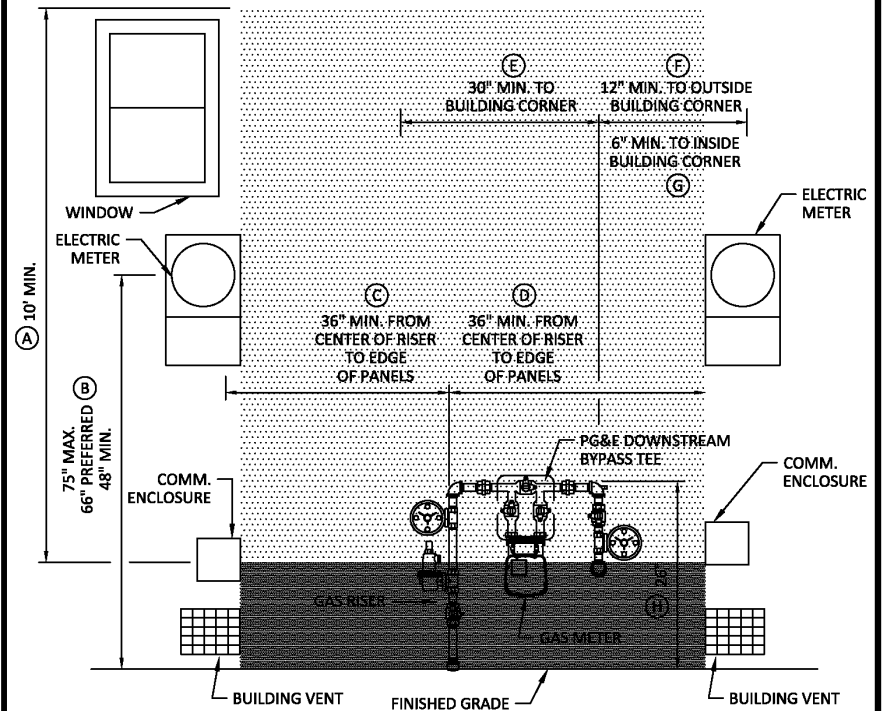
NATURAL GAS - FIGURE 09: GAS METER SET SEPARATIONS
