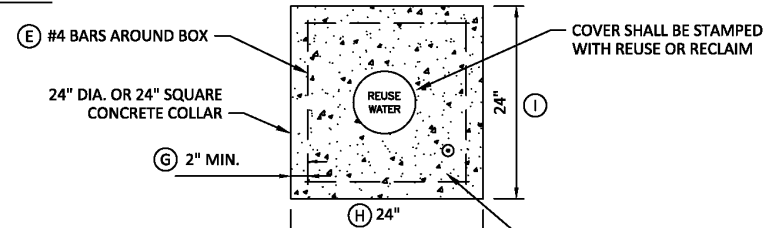
RW - FIGURE 04: VALVE & VALVE BOX DETAIL
