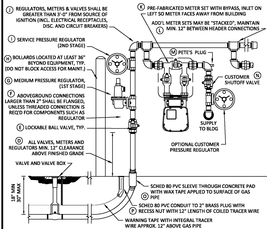
NATURAL GAS - FIGURE 07: MULTIPLE DIAPHRAGM GAS METER DETAIL Rev. 7/1/2019
