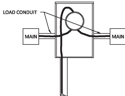
UNACCEPTABLE CONFIGURATION
