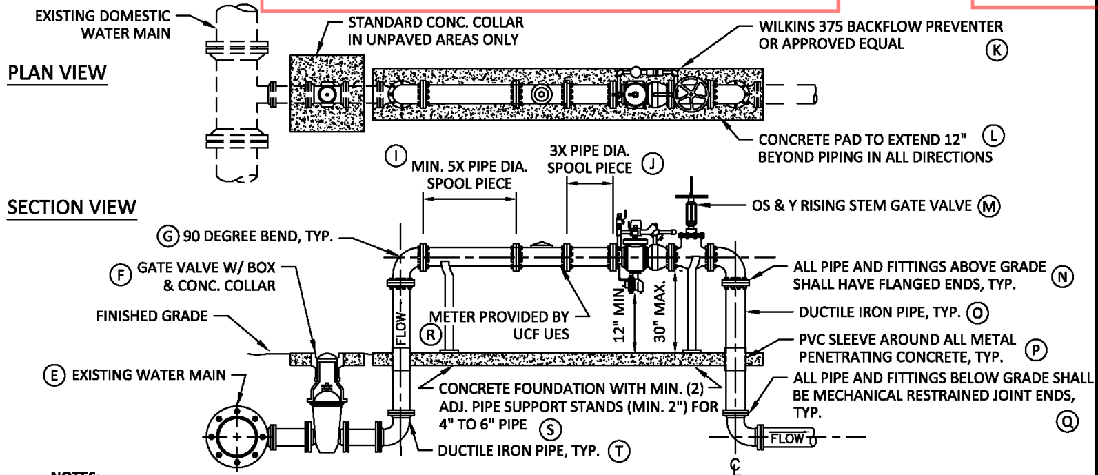
DW - FIGURE 07: 3" AND LARGER DOMESTIC WATER METER
