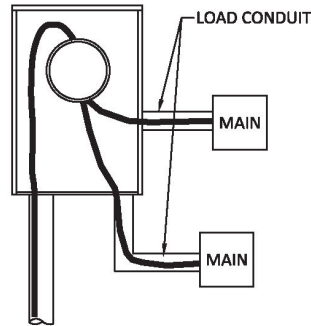
ACCEPTABLE CONFIGURATION
