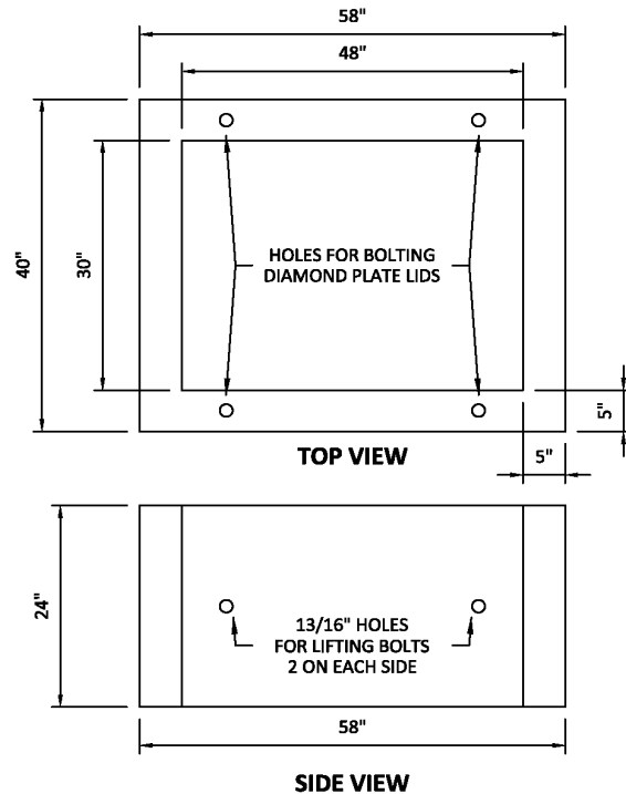
FIGURE 14A: SMALL PULL AND SPLICE BOX
