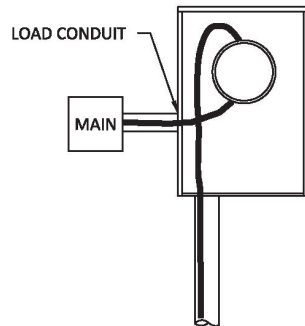
UNACCEPTABLE CONFIGURATION
