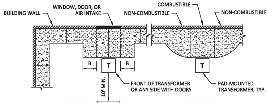
FIGURE 1 ALLOWABLE CLEARANCES
