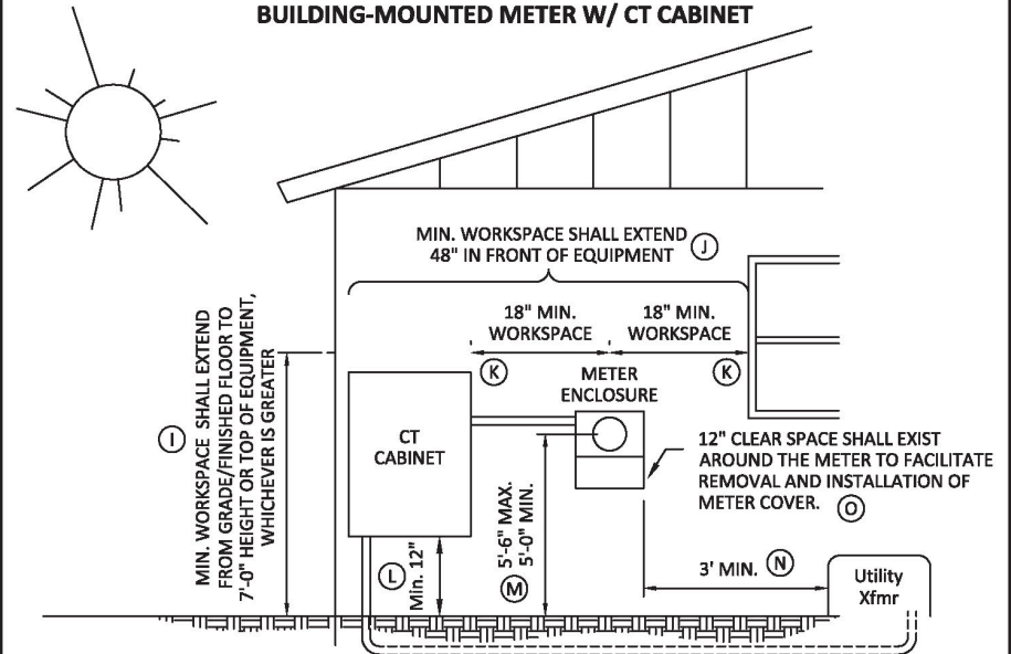
FIGURE 03C:
