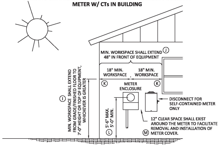
FIGURE 03B:
