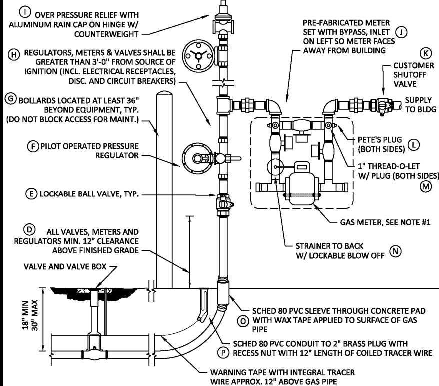
NATURAL GAS - FIGURE 06: SINGLE ROTARY GAS METER DETAIL Rev. 7/1/2019
