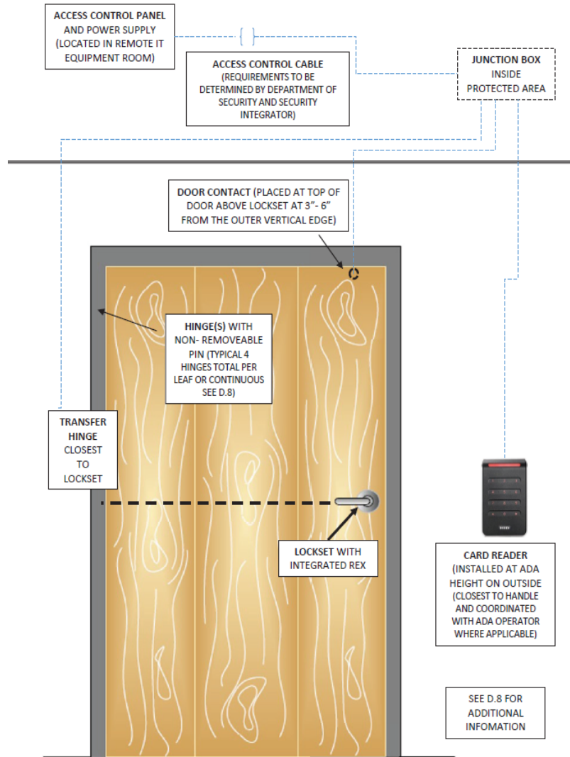
FIGURE 28-01 ACCESS CONTROL INSTALLATION DIAGRAM
