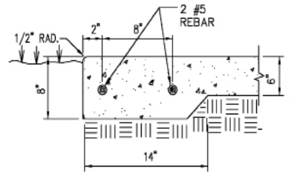
UP TO 10' WIDE CONC. WALK – THICKENED EDGE Concrete Walk Edge
