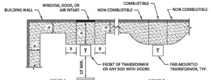
FIGURE 1 ALLOWABLE CLEARANCES
