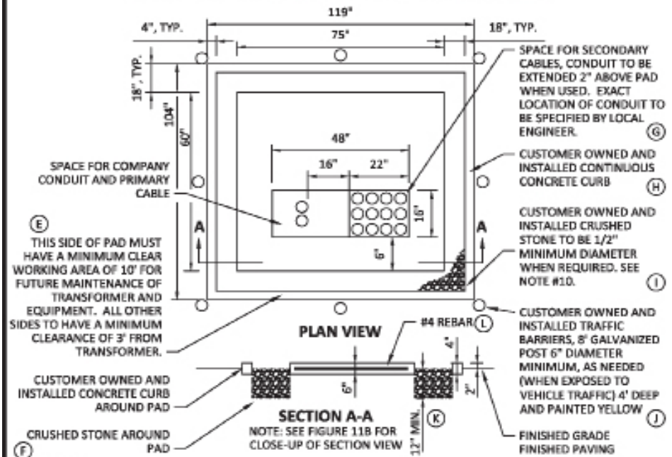
FIGURE 11A: 25 TO 300 KVA, 3 PHASE PADMOUNTED TRANSFORMERS
