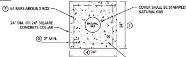
NATURAL GAS - FIGURE 04: VALVE & VALVE BOX DETAIL
