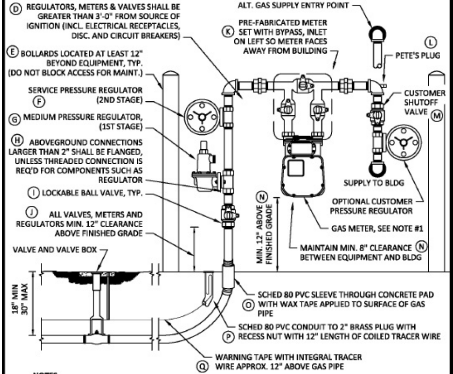
NATURAL GAS - FIGURE 05: SINGLE DIAPHRAGM GAS METER DETAIL
