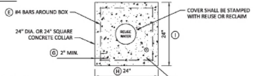
RW - FIGURE 04: VALVE & VALVE BOX DETAIL
