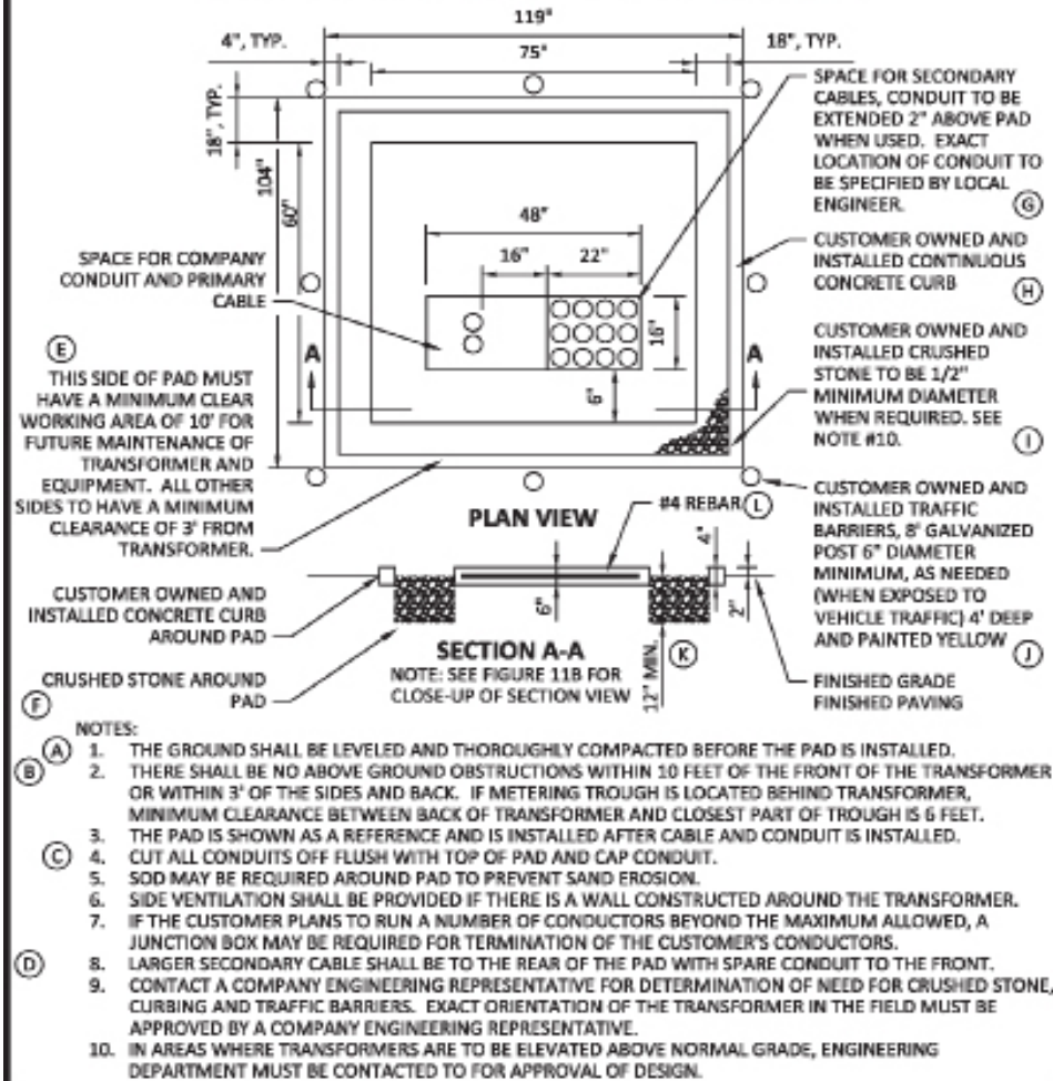
FIGURE 11A: 25 TO 300 KVA, 3 PHASE PADMOUNTED TRANSFORMERS
